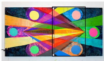
The Universe II
